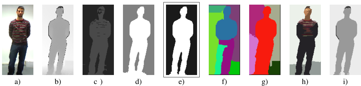
Fig. 10. Segmentation of the datasets acquired by the trinocular setup on a person scene. The figure shows: a) color image; b) corresponding depth-map; c) segmentation on the basis of color information only; d) segmentation on the basis of geometry only; e) segmentation based on the proposed method, fusing geometry and color; f) segmentation obtained by applying [1] to color information; g) segmentation obtained by applying [1] to geometry information; h) segmentation obtained by applying [27] to color information; i) segmentation obtained by applying [27] to geometry information;
