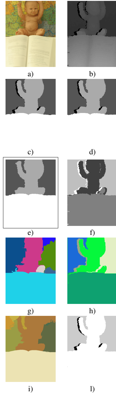
Fig. 12. Segmentation of the baby2 scene from the Middlebury dataset: a) color image; b) corresponding disparity map (disparity values have been stretched in order to improve the readability of the printed picture); c) segmentation based on the proposed method exploiting geometry and only one of the color views; d) segmentation based on the proposed method exploiting both color views and geometry as described in Section V; e) segmentation based on the proposed method exploiting both color views and geometry and also the occlusion handling scheme of Appendix A; f) segmentation performed by [17] that jointly exploits color and depth data; g) segmentation performed by [1] on the basis of color information only; h) segmentation performed by [1] on the basis of depth information only; i) segmentation performed by [27] on the basis of color information only; l) segmentation performed by [27] on the basis of depth information only.
